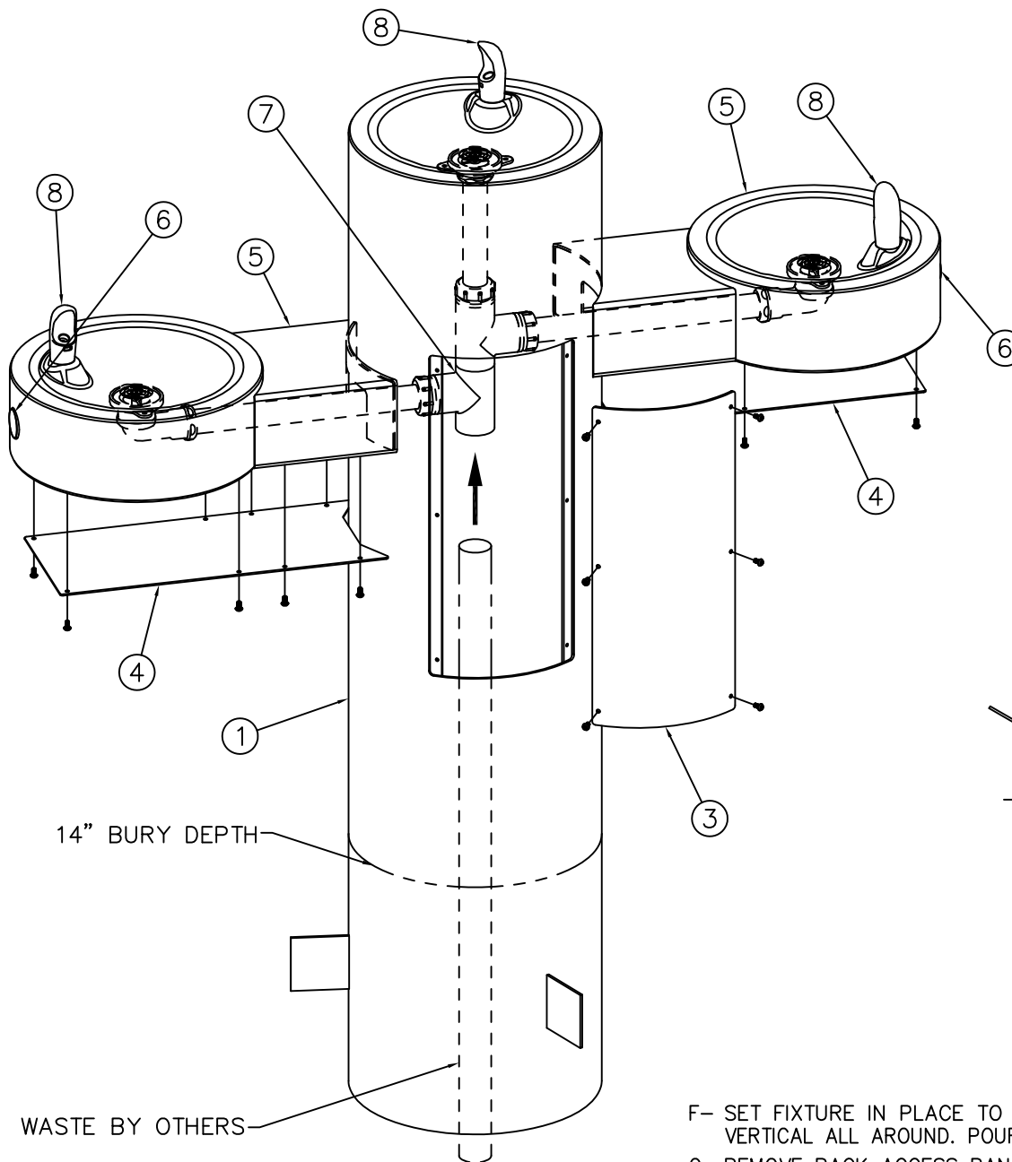
BASE ROUGH-IN VIEW
