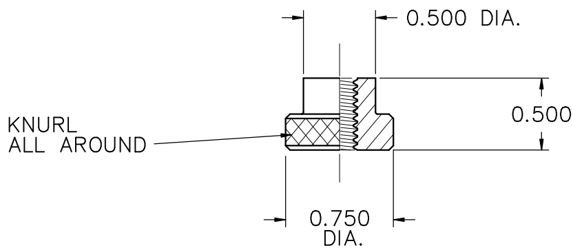
SECTION A
