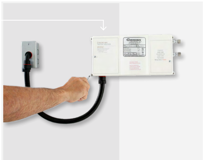
Replace cover on the tankless electric water heater.
