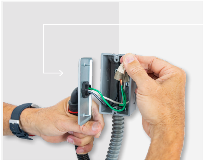
Install the Chronomite Tankless Electric Water Heater on the wall. Connect the end of the cord with the plate into the J-box on the wall.
