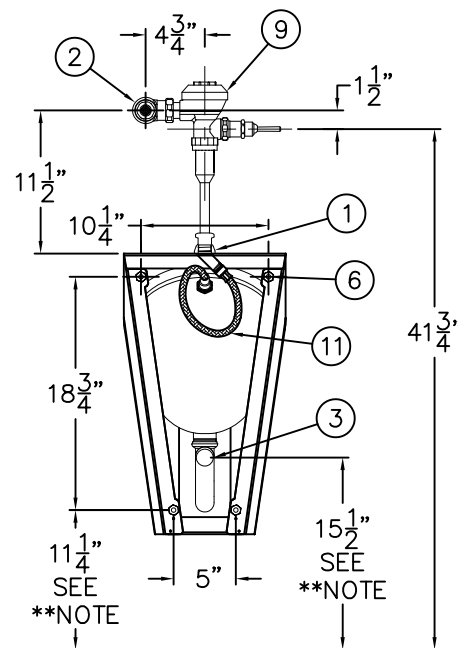
-T TOP SUPPLY REAR VIEW
