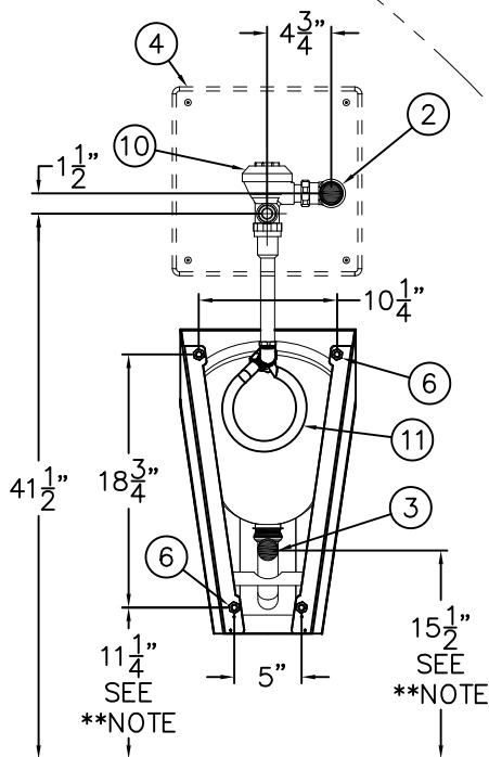
-W WALL SUPPLY REAR VIEW
