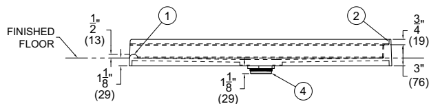
SIDE VIEW OF ADA BASE DETAIL NOT TO SCALE
