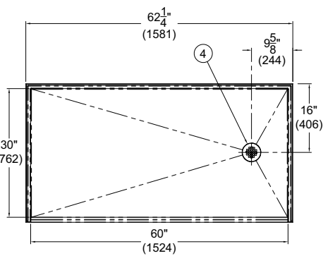
CSB6030ADA-R (CSB6030ADA-L OPPOSITE)
