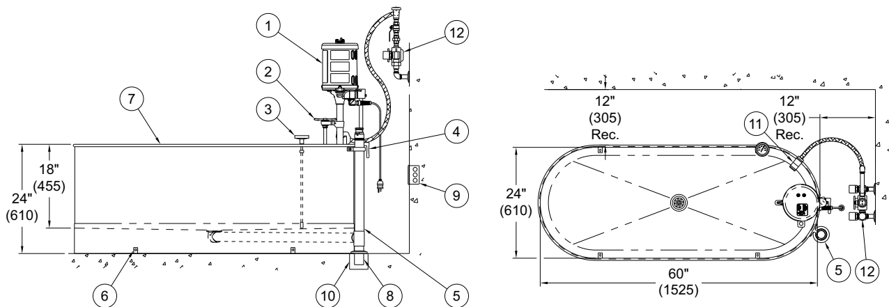
STATIONARY L-90-S SERIES WHIRLPOOL
