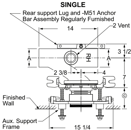
Fig. 0211RY-M54-XK Top View
