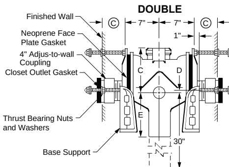
Fig. 0230D Side View
