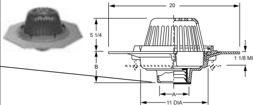
FIG. DX1010 WIDE FLANGE BODY - SECURED DOME
