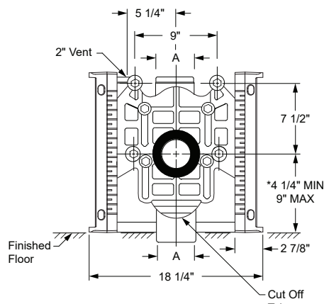
Fig. 0250Y-M54-XX Front View
