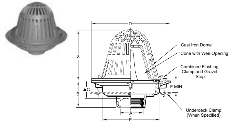
FIG. 1083 RAINTR® ROOF DRAINS
