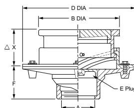
Fig. 4318 Heavy Duty Top
