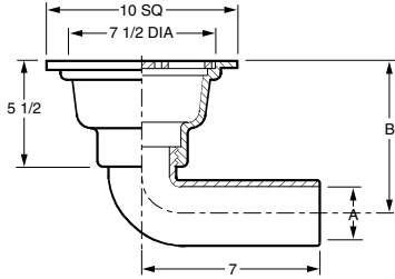
FIG. 2285 LIGHT DUTY FLOOR DRAIN WITH HINGED GRATE
