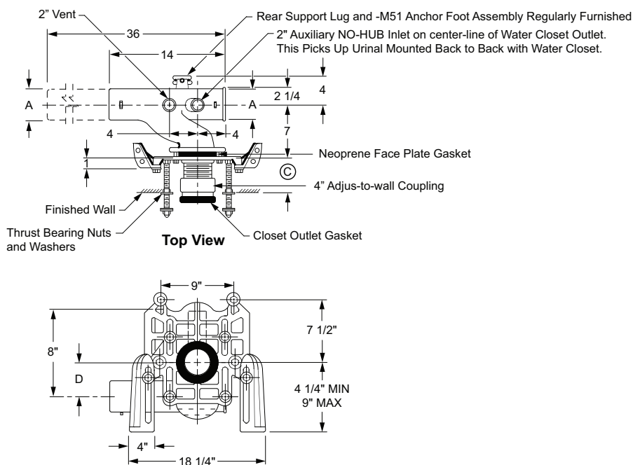
Fig. 0209Y Front View
