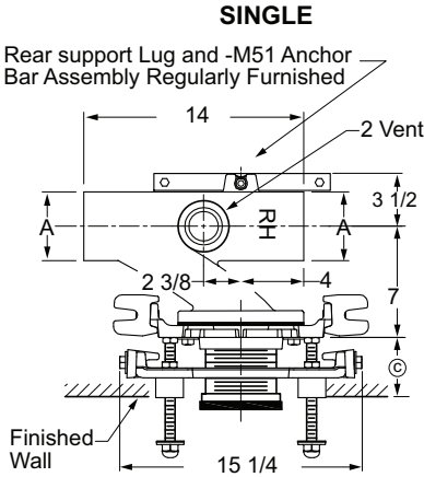
Fig. 0211RY-M58-M54-XK Top View
