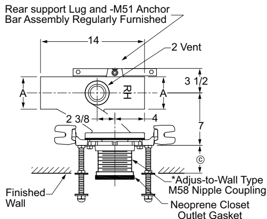
Fig. 0211RY-M58/M54-XX Top View
