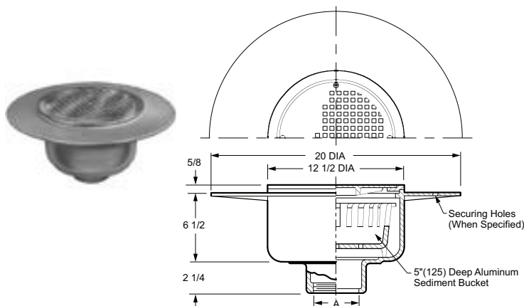
FIG. DX3068 SANI-CEPTOR® ARC FLOOR & INDIRECT WASTE DRAINS, WIDE FLANGE, ROUND NICKEL BRONZE TOP
