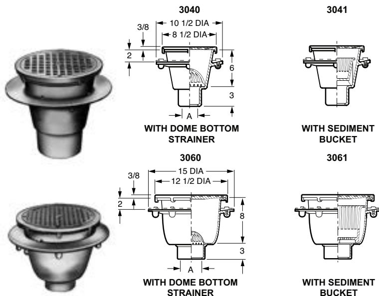
FIG. 3040 SERIES SANI-CEPTOR® ARC FLOOR & INDIRECT WASTE DRAINS, SHALLOW RECEPTOR, ROUND NICKEL BRONZE TOP FIG. 3060 SERIES SANI-CEPTOR® ARC FLOOR & INDIRECT WASTE DRAINS, SHALLOW RECEPTOR, ROUND NICKEL BRONZE TOP
