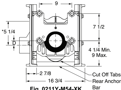
Fig. 0211Y-M54-XK Front View
