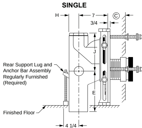
Fig. 0230Y-M54-XX Side View
