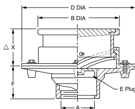
Fig. 4313 Medium Duty Top
