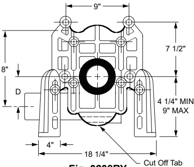
Fig. 0208RY Front View
