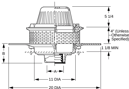
FIG. 1018 IRMA ROOF APPLICATIONS
