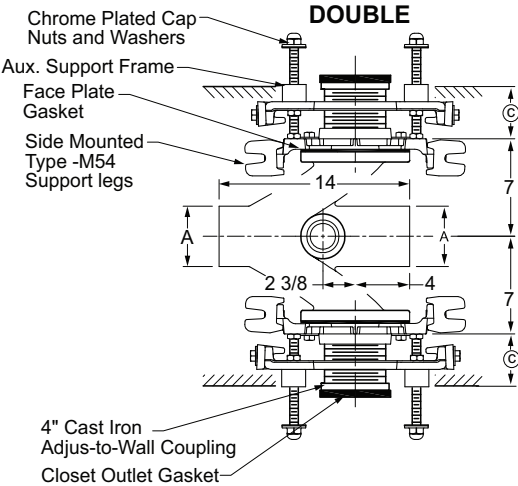
Fig. 0211DY-M58-M54-XK Top View
