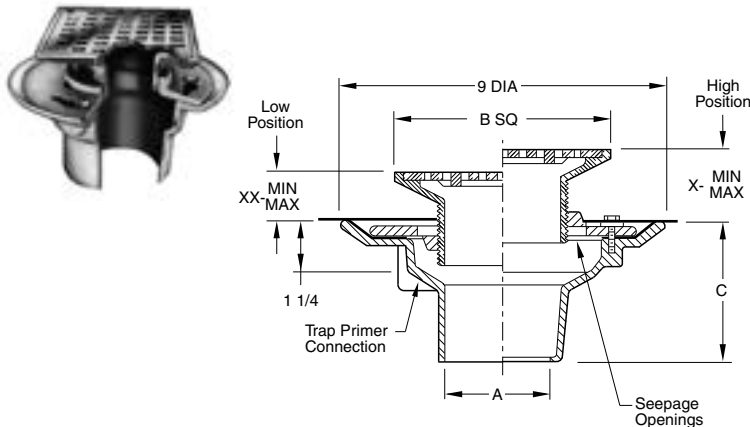
FIG. 2005 (-B) FLOOR DRAIN WITH ADJ. SQUARE STRAINER FIG. 2010 (-B) FLOOR DRAIN WITH ADJ. SQUARE STRAINER
