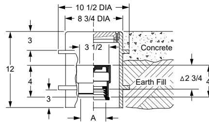
4250 Series 2" & 5" Sizes
