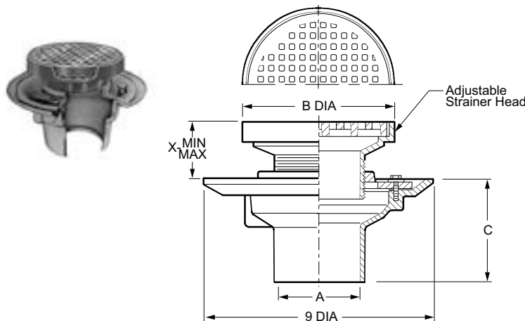
FIG. 2005(-D) FLOOR DRAIN AND ADJ. STRAINER WITH ROUND REINFORCED TRACTOR GRATE FIG. 2010(-E) FLOOR DRAIN AND ADJ. STRAINER WITH ROUND REINFORCED TRACTOR GRATE
