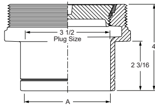
4280 Series 2" - 5" Sizes
