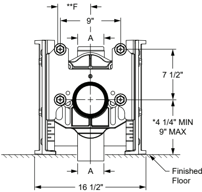
Fig. 0240Y-M58-M54-XK Front View
