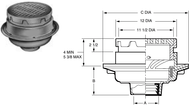
FIG. 2340 HEAVY DUTY FLOOR DRAIN WITH 12" ROUND ADJUSTABLE TOP AND TRACTOR GRATE
