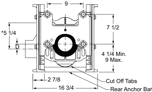
Fig. 0211Y-M58-M54-XK Front View
