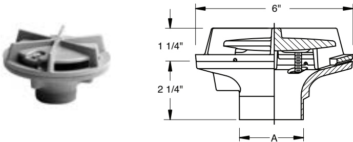
FIG. 1605 6" DIAMETER LOW PROFILE SIPHONIC GUTTER DRAIN
