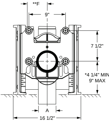
Fig. 0230Y-M58-M54-XK Front View
