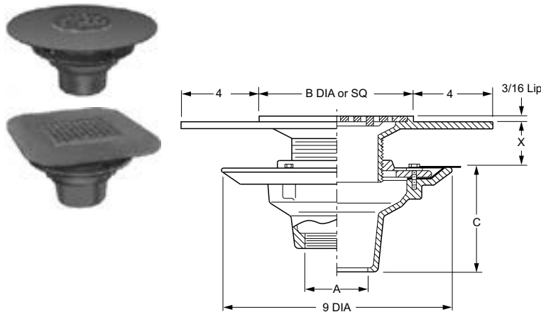
FIG. DX2005 (A) FLOOR OR SHOWER DRAIN AND ADJ. WIDE FLANGE STRAINER WITH ROUND GRATE FIG. DX2010 (B) FLOOR OR SHOWER DRAIN AND ADJ. WIDE FLANGE STRAINER WITH SQUARE GRATE
