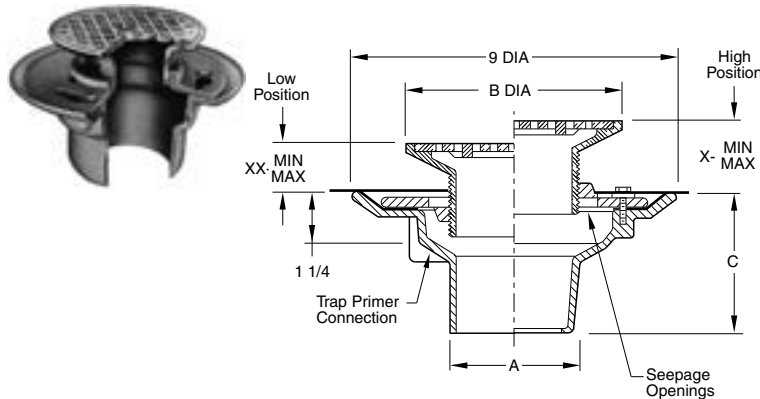
FIG. 2005 (-A) FLOOR DRAIN WITH ADJ. ROUND STRAINER FIG. 2010 (-A) FLOOR DRAIN WITH ADJ. ROUND STRAINER
