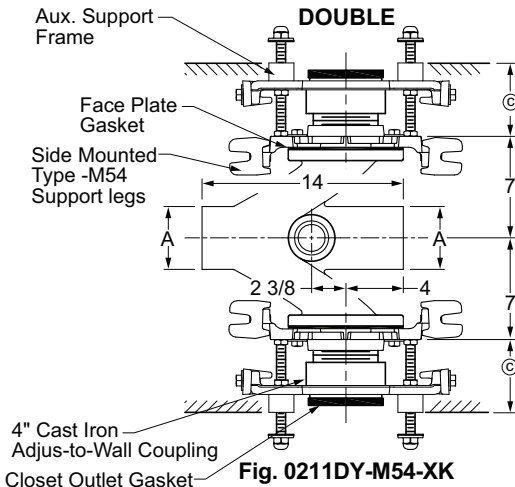
Fig. 0211DY-M54-XK Top View
