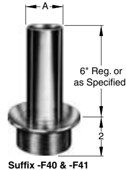
FIG. 3580, 3581, 3590, 3591 FUNNEL ASSEMBLIES ONLY
