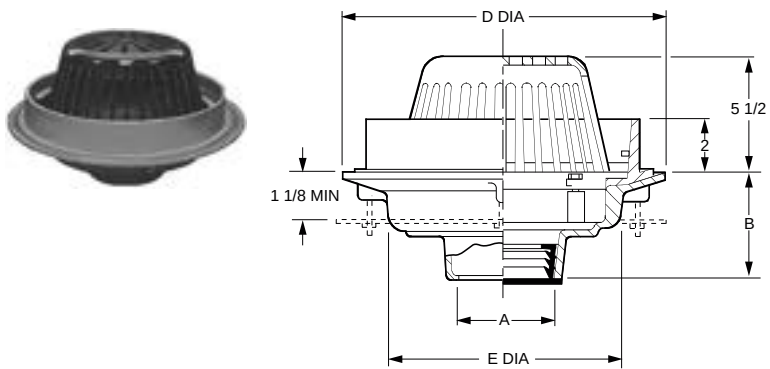
FIG. 1080 SPECIAL PURPOSE ROOF DRAINS WATER DAM TYPE
