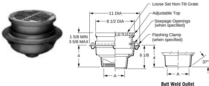
FIG. 9725 FLOOR DRAIN WITH 8 1/2" ROUND ADJUSTABLE TOP
