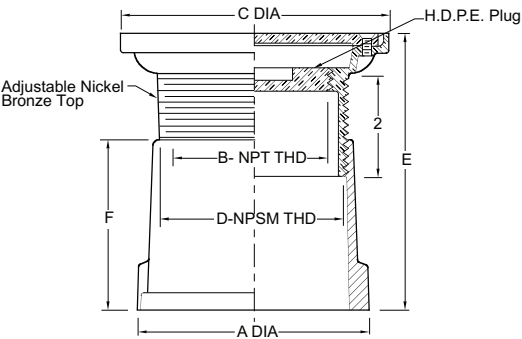
FIG. 4429 ROUND ADJUSTABLE NICKEL BRONZE TOP
