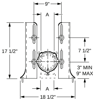
Fig. 0548F Front View
