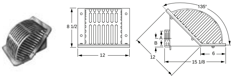
FIG. 1580 SCUPPER DRAIN - CONVEX GRATE
