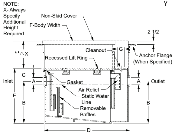
Side View Fig. 8450E Shown
