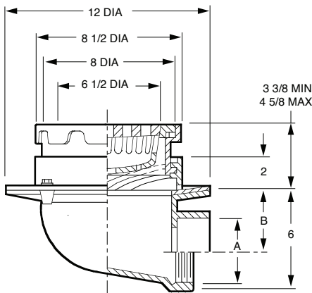
FIG. 2355 FLOOR DRAIN WITH 8 1/2" ROUND ADJUSTABLE TOP AND "SAFE-SET®" SEDIMENT BUCKET
