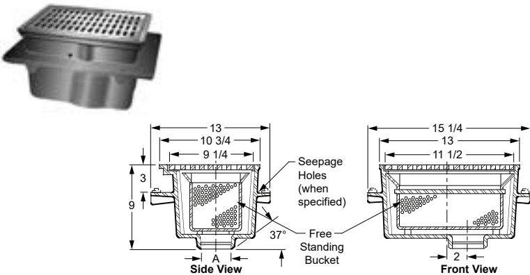
FIG. 9755 SQUARE HEAVY DUTY DRAIN W/POLISHED BRONZE TOP AND FREE STANDING SEDIMENT BUCKET
