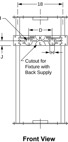
FIG. 0616, 0617 LABOR SAVER® OFF-THE-FLOOR URINAL SUPPORTS WITH HANGER PLATES FOR BLOWOUT AND WASHOUT URINALS WITH WALL HANGERS
