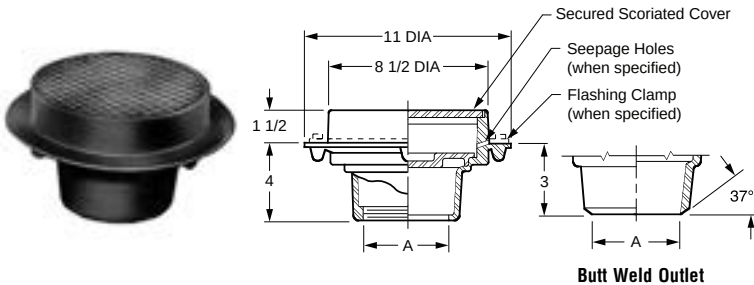
FIG. 9720 FLOOR DRAIN W/8 1/2" ROUND TOP, SOLID SCORIATED COVER AND CLOSURE PLUG
