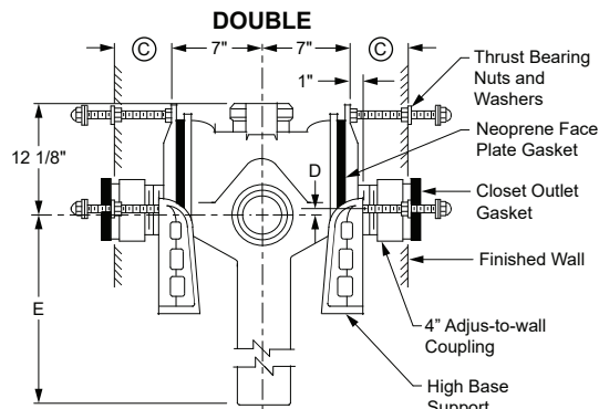
Fig. 0175D - 0185D Side View
