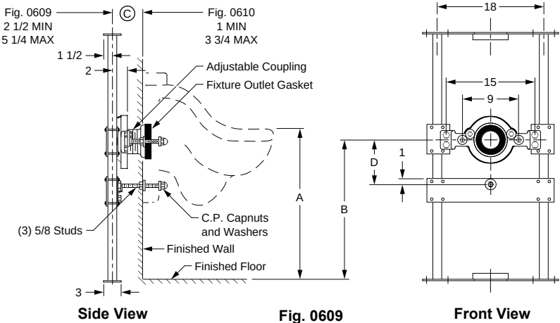
FIG. 0609, 0610 LABOR SAVER® OFF-THE-FLOOR URINAL SUPPORTS WITH SUPPORTING STUDS AND ADJUSTABLE COUPLING FOR BLOWOUT URINALS
