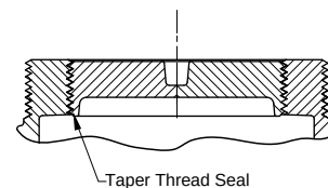
Fig. 11 Taper Thread Closure
