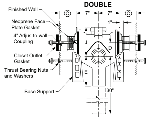
Fig. 0340D Side View
