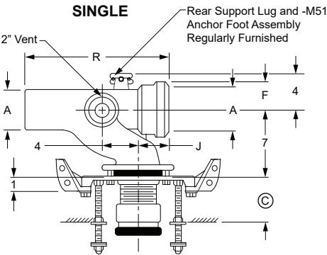
Fig. 0115R Top View
