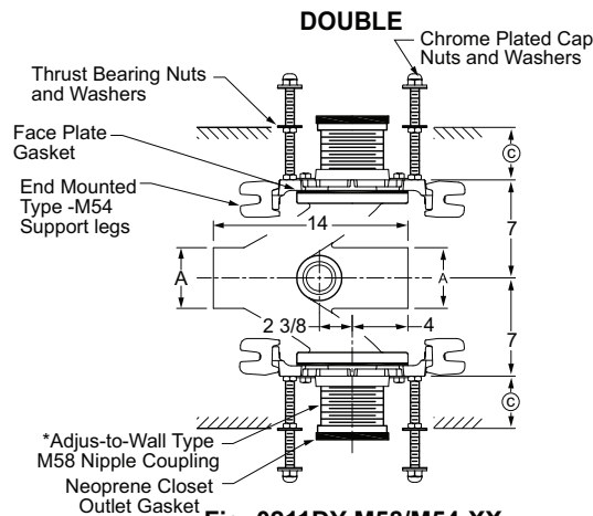
Fig. 0211DY-M58/M54-XX Top View
