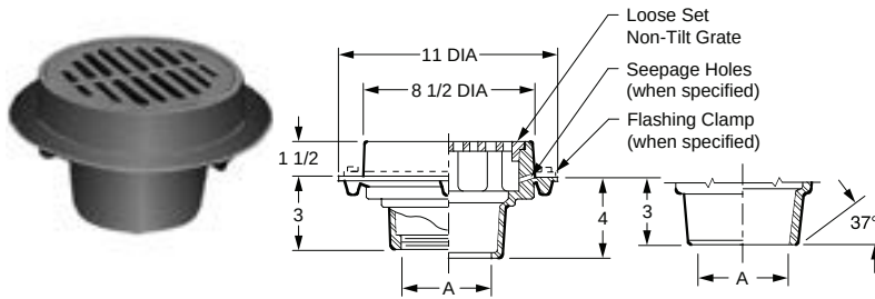
Butt Weld Outlet
