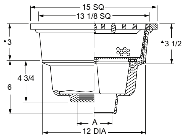
FIG. 2295 HEAVY DUTY FLOOR DRAIN
