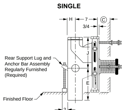
Fig. 0230Y-M58-M54-XX Side View
