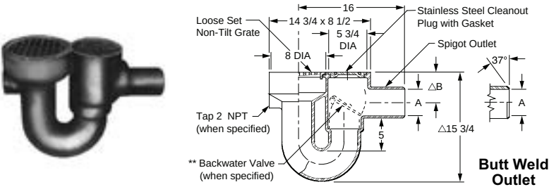
FIG. 9750 INTEGRAL TRAP DRAIN WITH FLOOR LEVEL CLEANOUT
