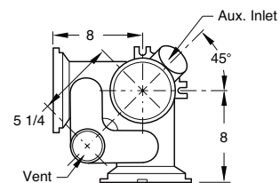
Fig. 0650Y Top View
