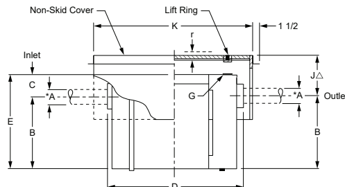
Side View Fig. 8335 Shown
