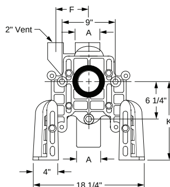
Fig. 0340Y Front View
