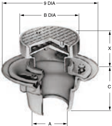
FIG. 2005 (-J) FLOOR DRAIN AND ADJ. STRAINER WITH ROUND SPANNER WRENCH COVER FIG. 2010 (-J) FLOOR DRAIN AND ADJ. STRAINER WITH ROUND SPANNER WRENCH COVER
