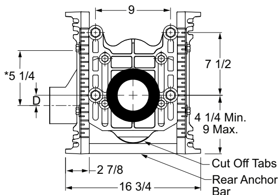
Fig. 0211Y-M58/M54-XX Front View
