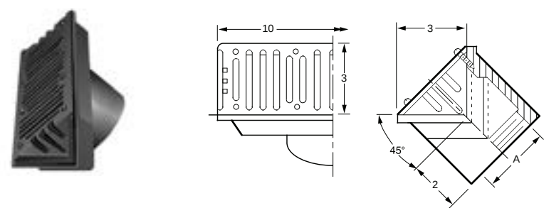
FIG. 1570 SCUPPER DRAIN - 45° OUTLET
