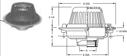
FIG. 1010 16" DIAMETER - LOW PROFILE DOME
