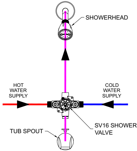
TYPICAL PIPING w/ TUB SPOUT
