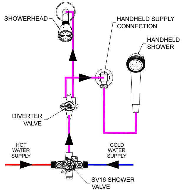
TYPICAL PIPING w/ HANDHELD SHOWER
