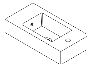
Model 9100-WM-H1R Micro Slab Deck Configured with Right Hand Faucet Hole
