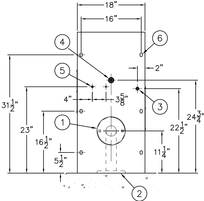
ROUGH-IN VIEW FROM FIXTURE SIDE OF LR1418FA-CT & LR1418FA-AR UNITS FOR FLOOR OR WALL OUTLET. LR1418FA-AL UNITS OPPOSITE.
