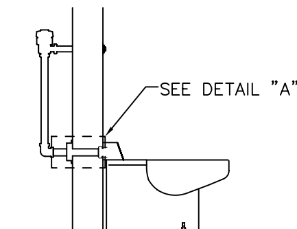
Toilet Flushing Inlet Connection
