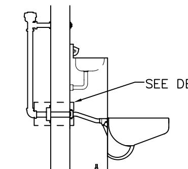
Comby Flushing Inlet Connection
