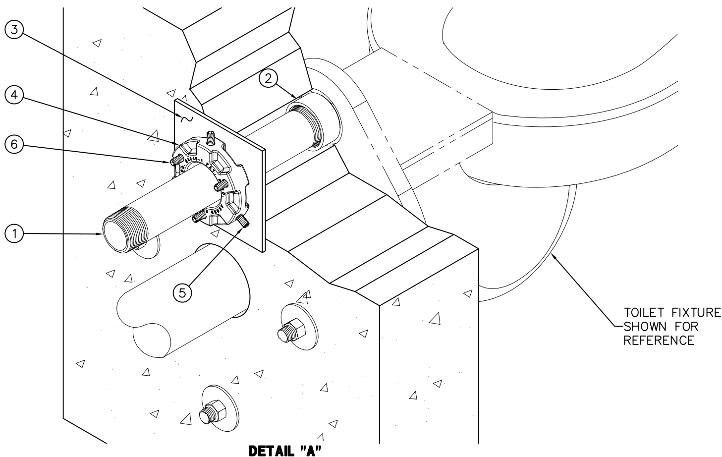
Lavy Waste Connection
